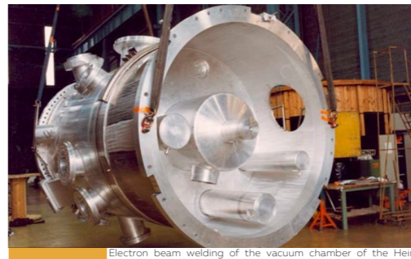
Electron beam welding of the vacuum chamber of the Heinz Maier-Leibnitz (FRM II) research reactor's neutron source
