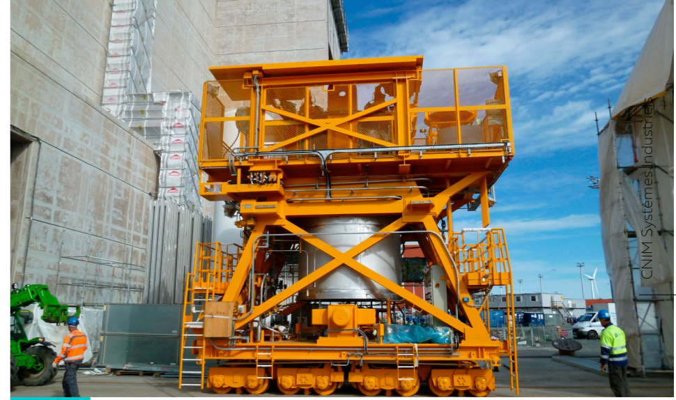
OL3 EPR spent fuel loading and unloading trolley in Finland
